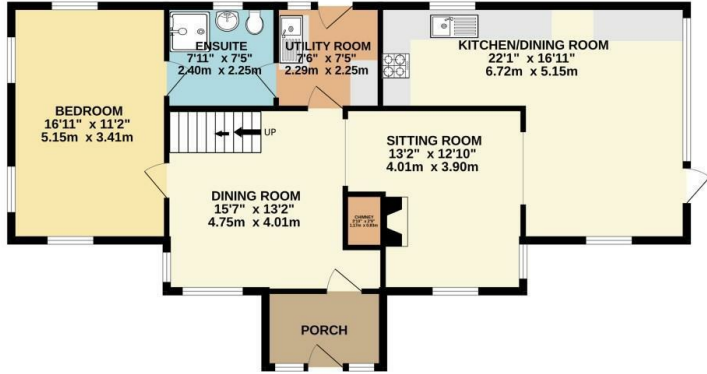
GROUND FLOOR 956 sq.ft. (88.8 sq.m.) approx.
